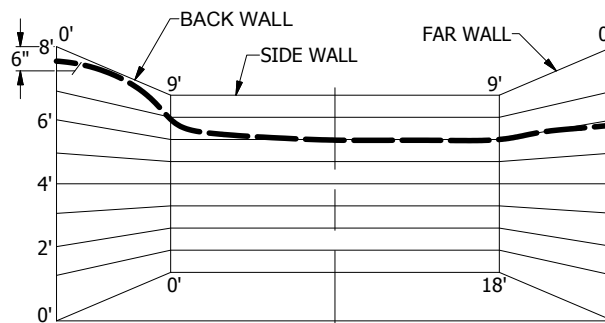
GL4234 - 22 GPM - 27.4 PSI DEFLECTOR 6" BELOW CEILING 18' x 18' ROOM SIZE (HALF PATTERN)
