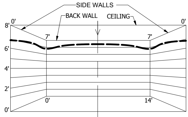
GL3511 & GL3547 - 11 GPM - 7.2 PSI 14' x 14' ROOM SIZE (HALF PATTERN)
