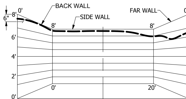
GL4234 - 27 GPM - 41.3 PSI DEFLECTOR 6" BELOW CEILING 16' x 20' ROOM SIZE (HALF PATTERN)
